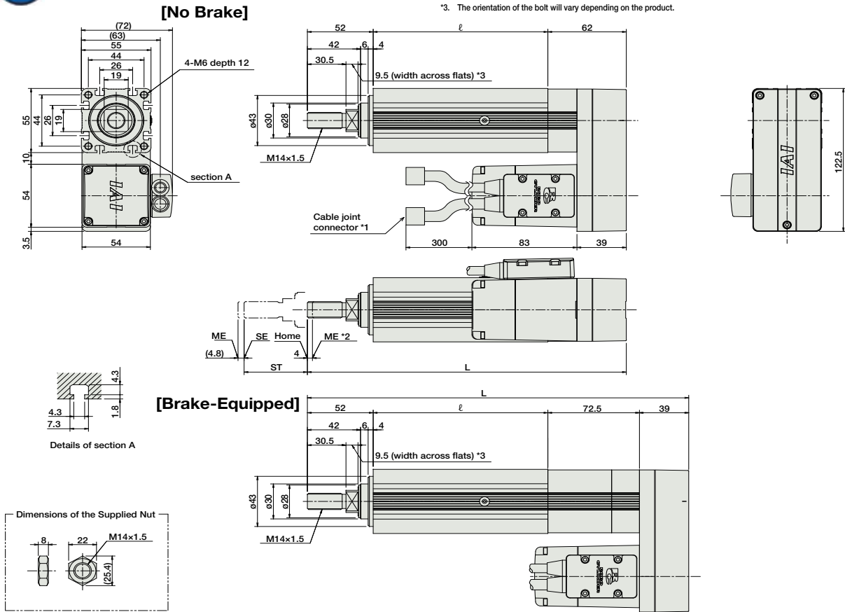
RCS2-RA5R (without brake)
