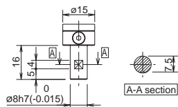
Detail view of vertical axis tip (*3)
